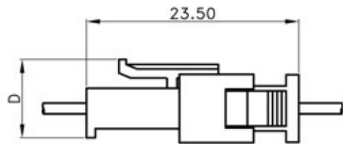
Assembled Dimension
