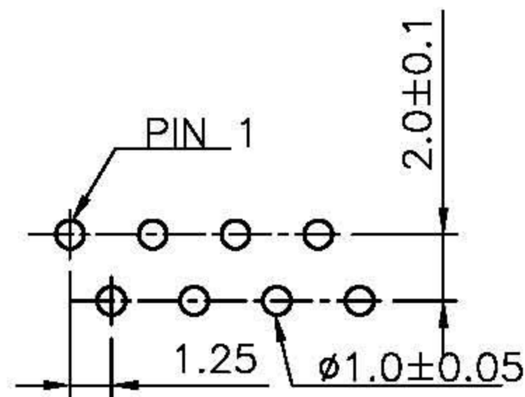
Recommmand PCB Layout
