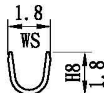
B-B Section
